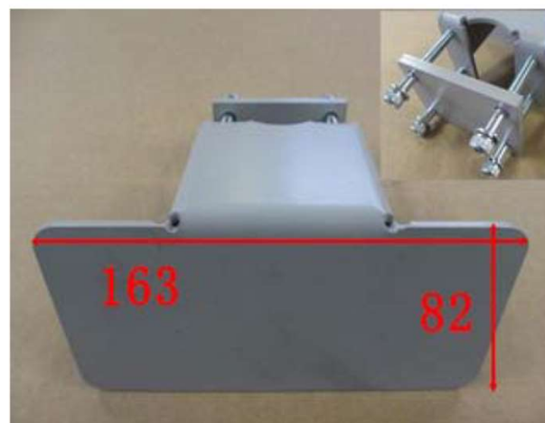
BM8-3 Foot Guard Assy
