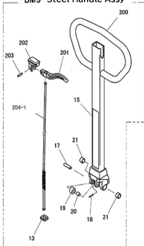
BM9 Steel Handle Assy
